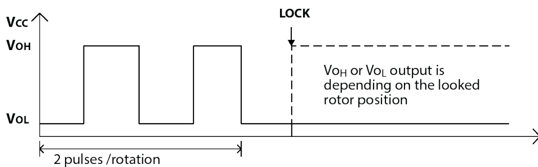
Output Waveform
